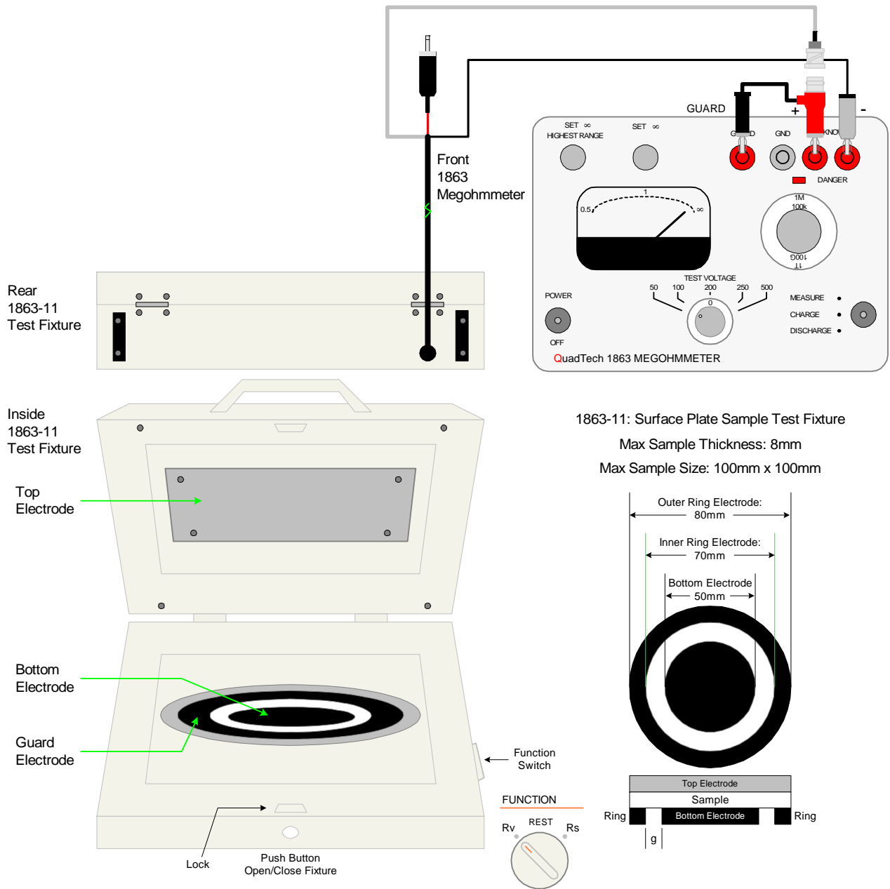
Figure 2: Connection of an 1863-11 Test Cell to an 1863 Megohmmeter
