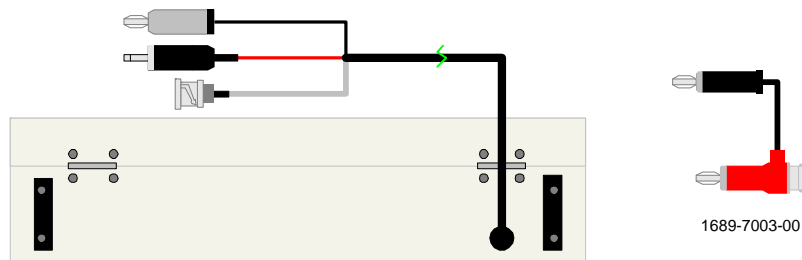
Figure 1: Rear View of 1863-11 Test Cell
